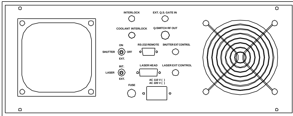
Fig. LC-100 rear panel
